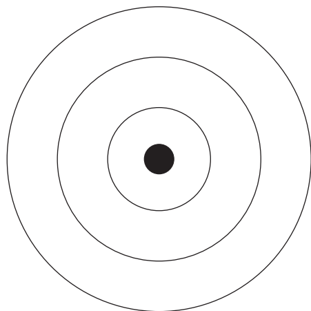
Magnesium atom
