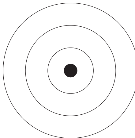
Chlorine atom
